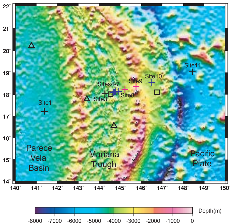
Fig. 1 Locations of ocean bottom electro-magnetic field observation sites in the central Mariana area. Black crosses, OBEM recovered during the KR02-14 cruise; red crosses, OBEM recovered during a R/V Ewing cruise (Goto et al., 2002b); blue crosses, OBEM not recovered during the KR02-14 cruise; triangles, electro-magnetic field observation sites of the Ocean Hemisphere Project, Japan (Seama et al., 2000); squares, electro-magnetic field observation sites by Filloux (1987). Color image of bathymetry map is from Smith and Sandwell (1994).
