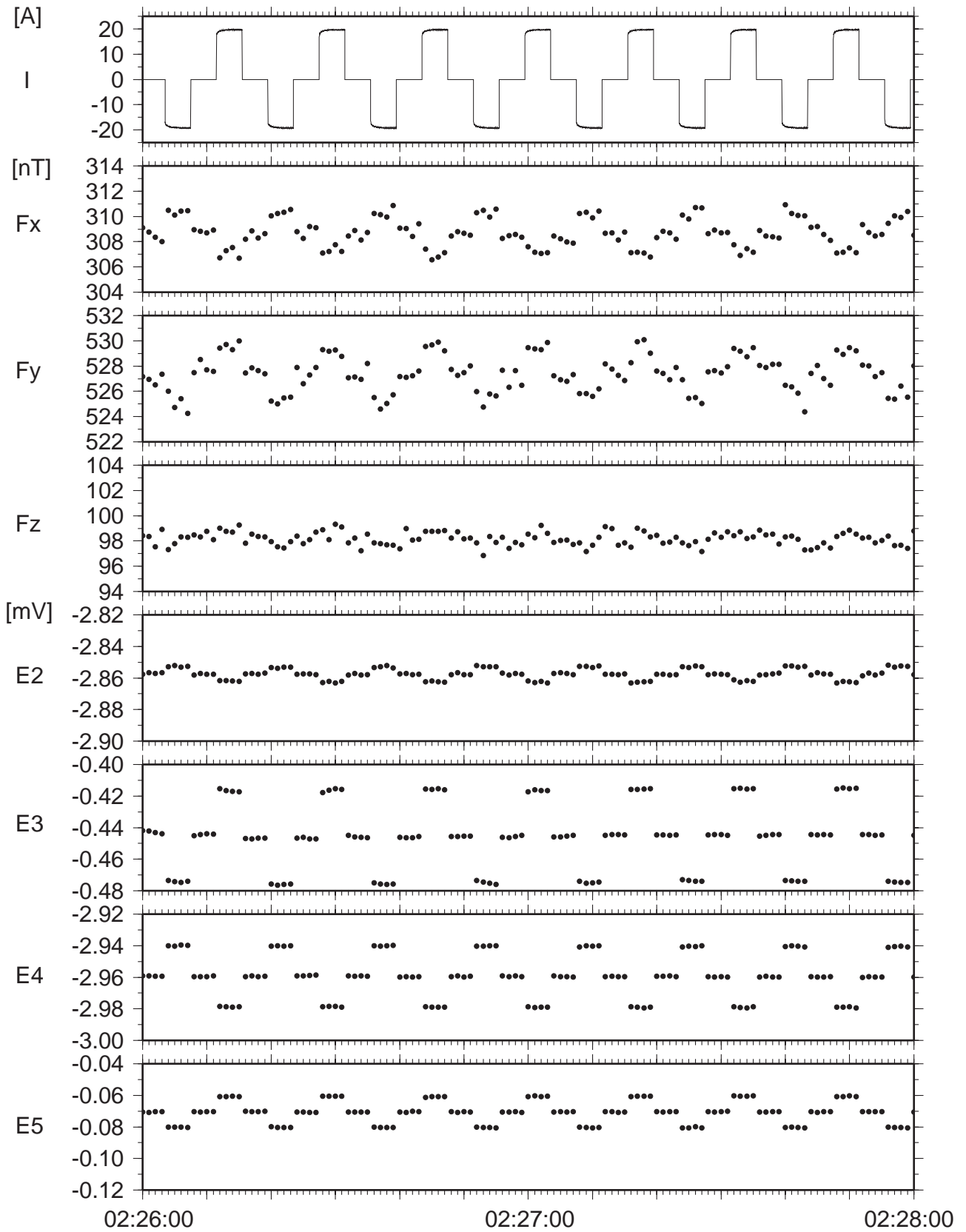
Fig. 11 An example of data obtained by the MMR experiment. "I" indicates time series of the electric current data supplied by the onboard unit. F_x and F_y show magnetic field variations of two orthogonal horizontal components and F_z is that of downward component recorded by OBEM. E_2 , E_3 , E_4 and E_5 are the electric field variations obtained by four electrodes of OBEM with respect to the common electrode ( E_1 ).
