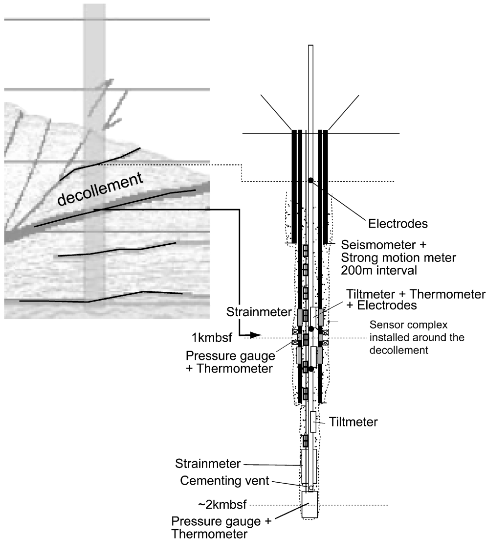
Fig. 5. Installation plan for sensors in a borehole near the décollement around the trench axis. Because crustal movement and fluid flow are expected near the décollement , the sensors should be deployed densely around the décollement .
