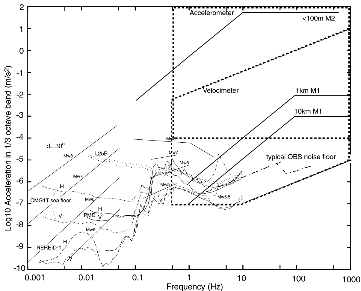
Fig. 2. Relation between frequency band and sensitivity in earthquake observation. Typical ambient noise spectra from broadband borehole seismometer in the Japan Trench (NEREID-1), broadband seismometer on the sea floor off Sanriku (CMG1T), and intermediate period seismometer on the sea floor (PMD) are plotted. Typical noise spectrum of a conventional OBS with short-period seismometer is also shown (L25B). H and V indicate vertical component and horizontal component of seismometer, respectively. The accelerations expected from earthquakes of different magnitudes at various epicentral distances are also shown by solid lines (Agnew et al. , 1986). Polygons with thick dash lines indicate frequency band and dynamic range of velocimeter and accelerometer for microearthquake observation in a deep borehole. Note that the noise level from sea floor borehole seismometer (denoted by NEREID-1) is lowest with a frequency band from 0.01 Hz to 10 Hz.
